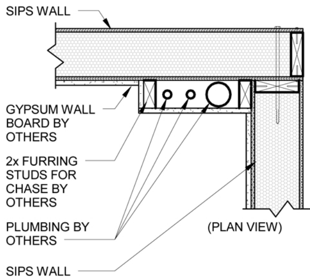
1 WALL CHASE @ CORNER D10 1" = 1'-0"
