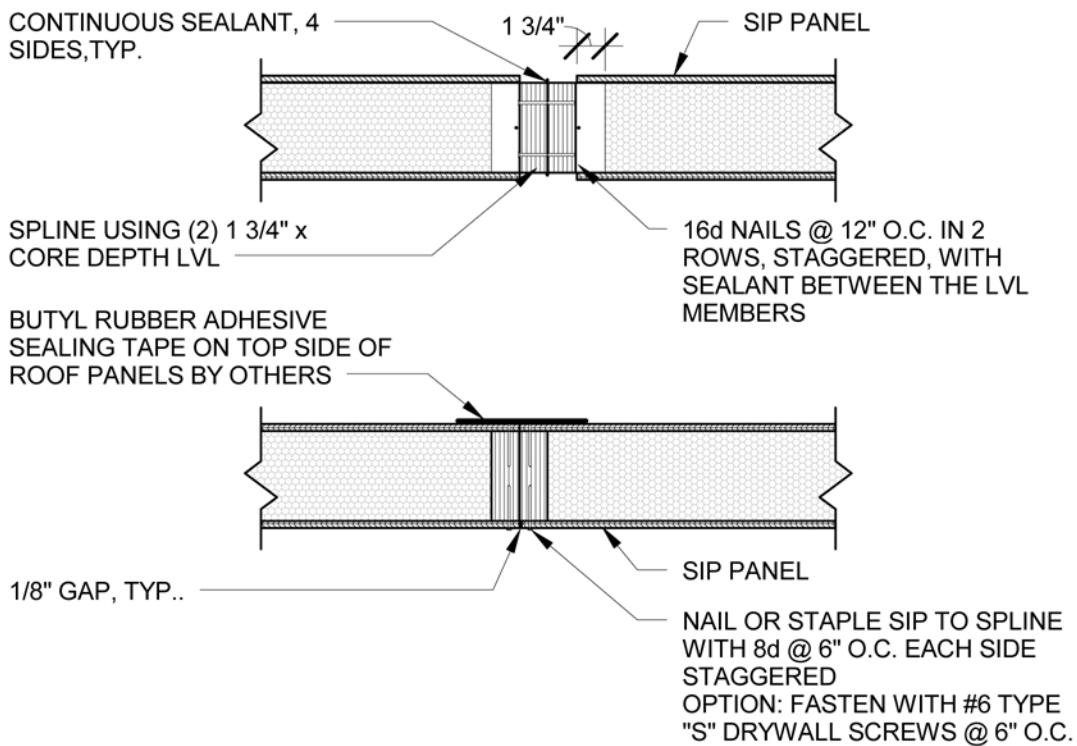
1 PANEL CONNECTION WITH LVL D12 1" = 1'-0"
