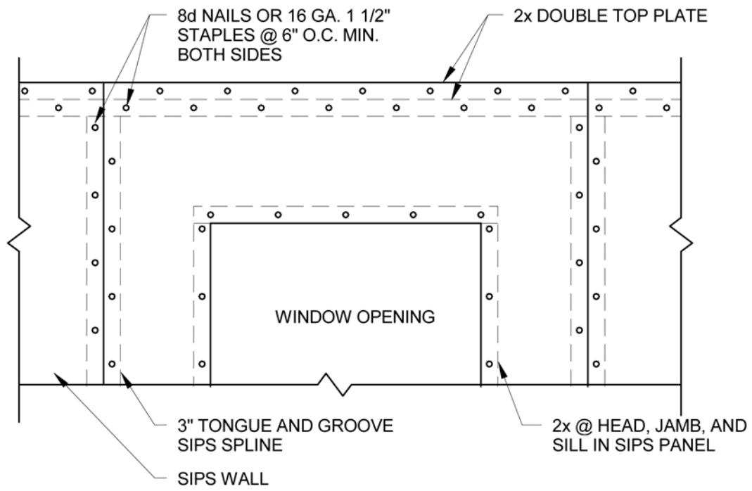
1 WINDOW OPENING IN PANEL D20 1" = 1'-0"
