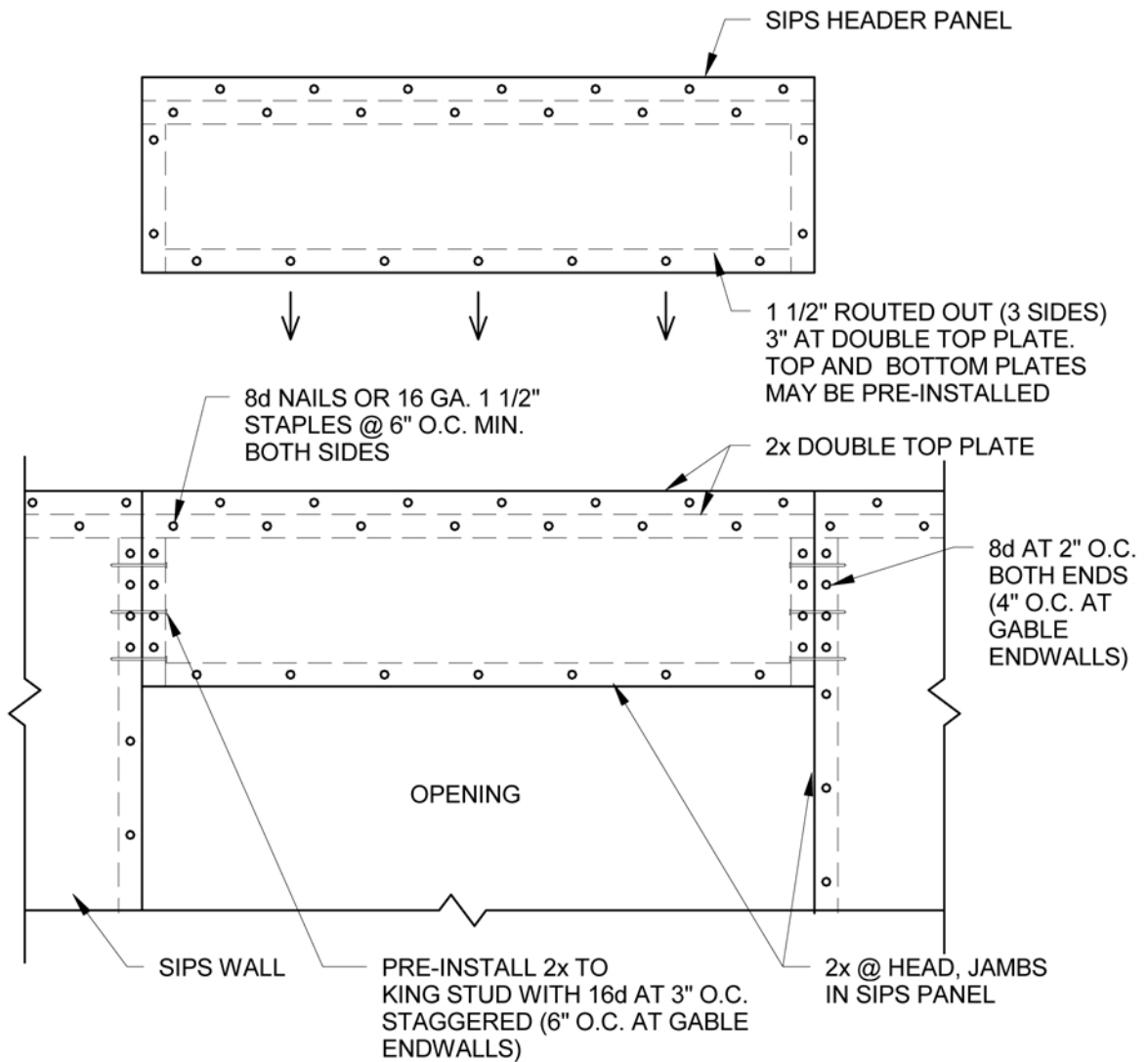
1 DISCONTINUOUS PANEL HEADER D21 1" = 1'-0"
