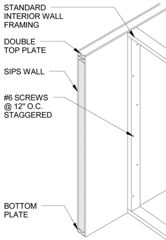
1 INTERIOR WALL CONNECTION D22 1/2" = 1'-0"
