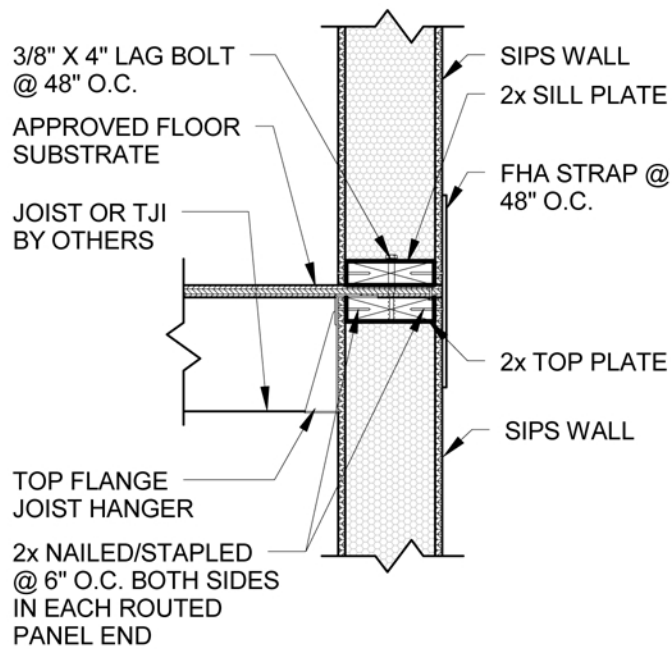
1 2-STORY WALL/FLOOR DETAIL D26 1" = 1'-0"
