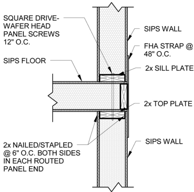
1 D27 2-STORY WALL/ SIPS FLOOR DETAIL 1" = 1'-0"
