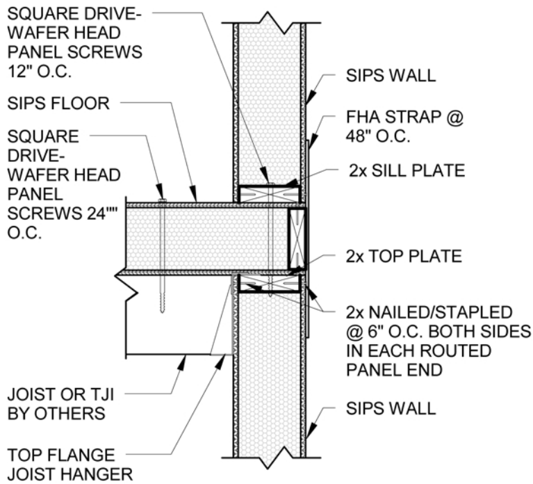
1 D28 2-STORY WALL/ SIPS/STRUCT FLOOR DETAIL 1" = 1'-0"
