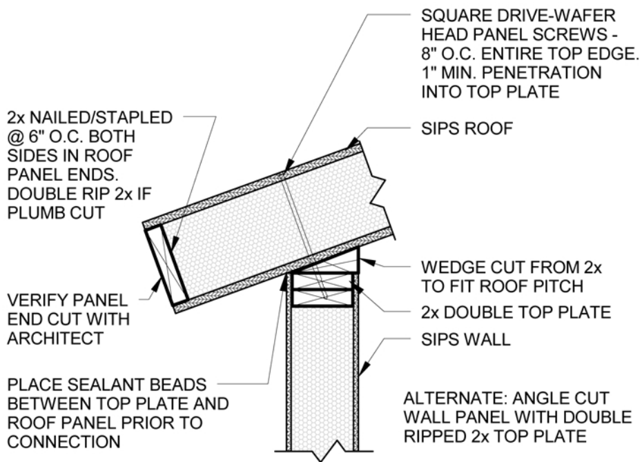
1 ROOF EAVE TO WALL CONNECTION D3 1" = 1'-0"
