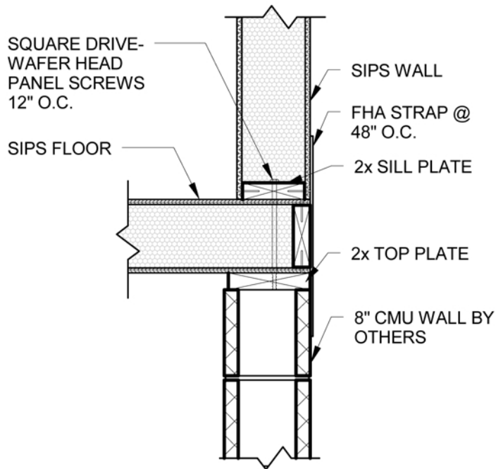
1 D30 2-STORY WALL/ SIPS FLOOR/CMU DETAIL 1" = 1'-0"
