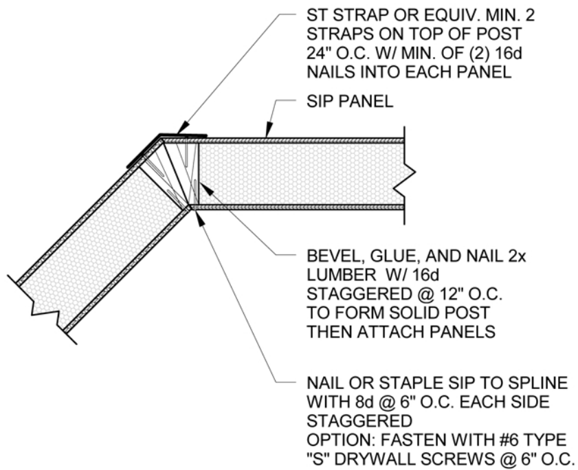
1 45 DEGREE POST DETAIL D31 1" = 1'-0"
