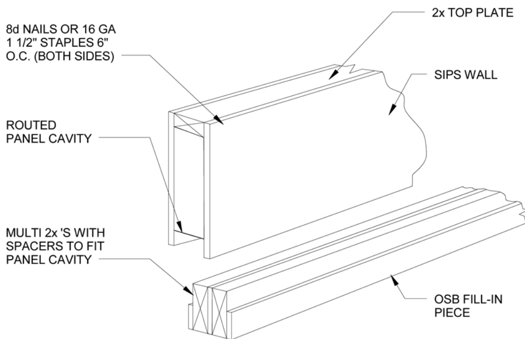
1 BUILT-UP HEADER DETAIL D33 1/4" = 1'-0"
