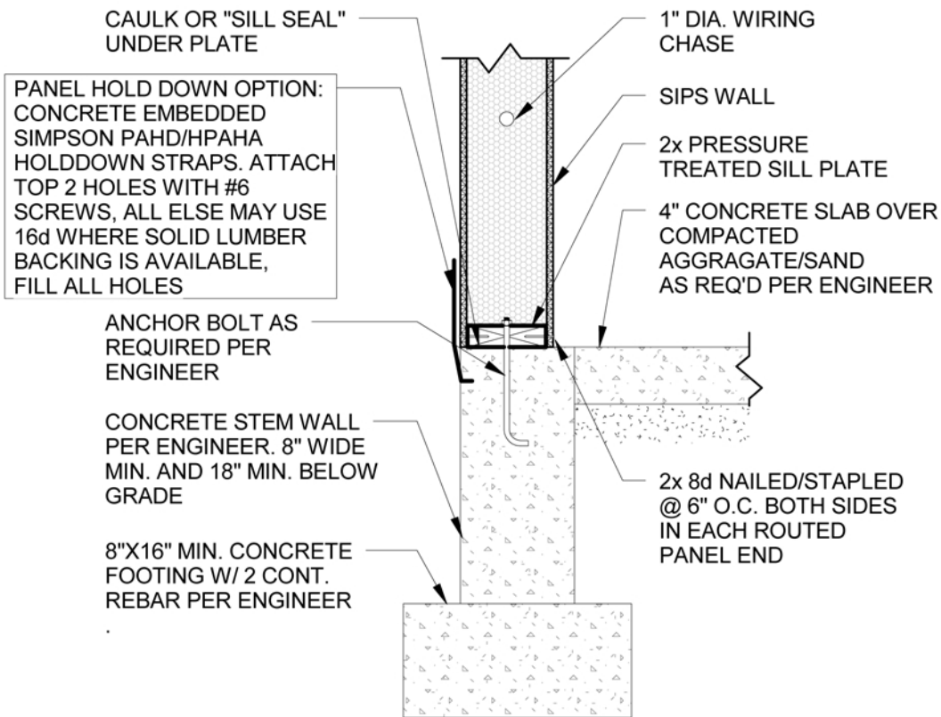
1 FOUNDATION DETAIL D36 1" = 1'-0"
