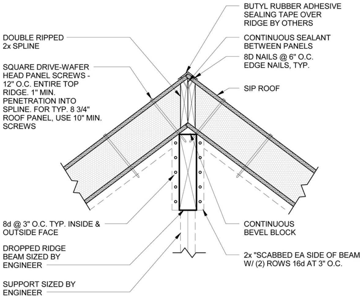
1 RIDGE BEAM @ END WALL D38 1" = 1'-0"
