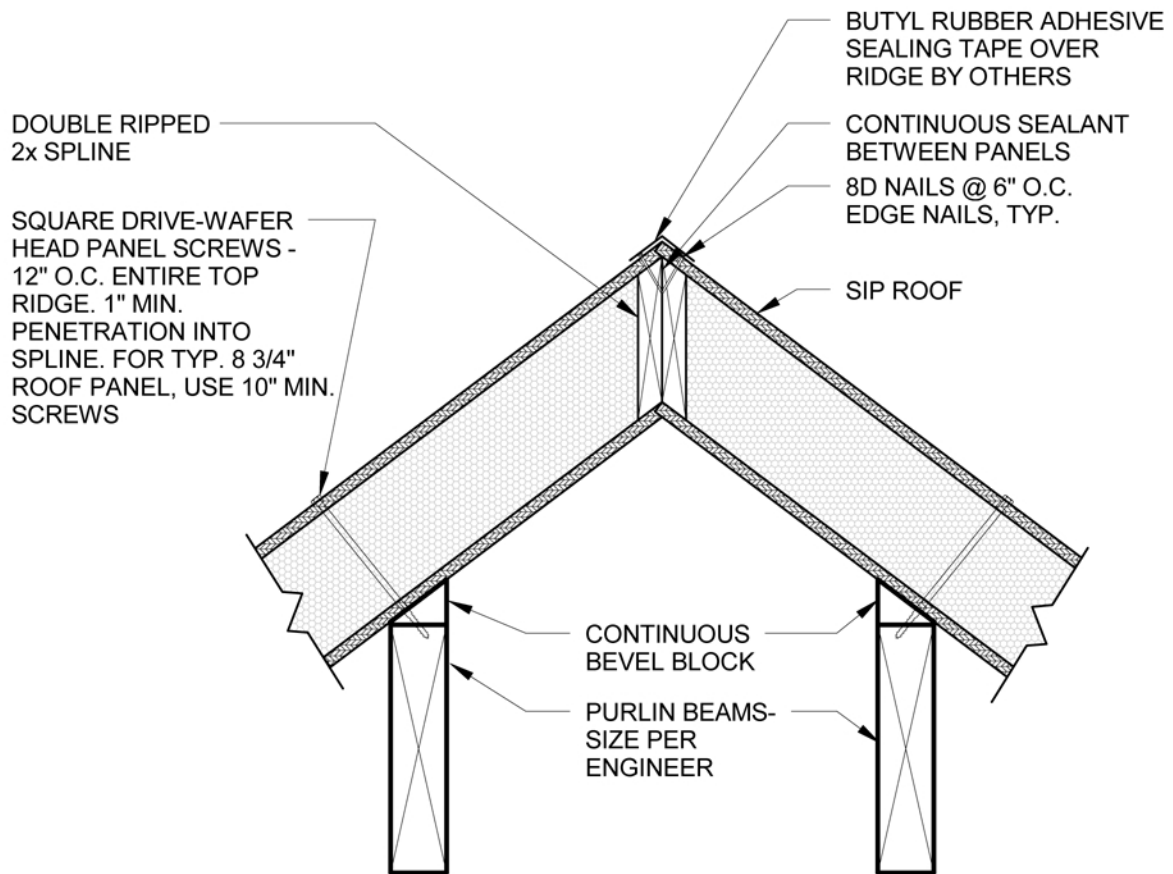
1 ROOF RIDGE W/ PURLINS D39 1" = 1'-0"
