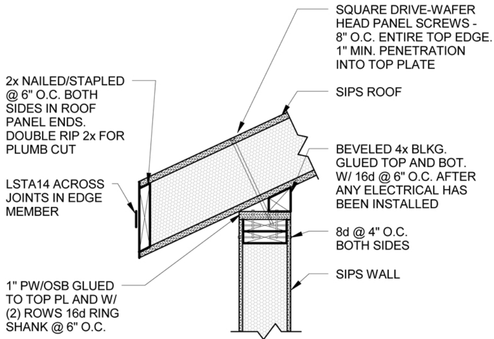
1 ROOF EAVE TO WALL CONNECTION ALT. D4 1" = 1'-0"
