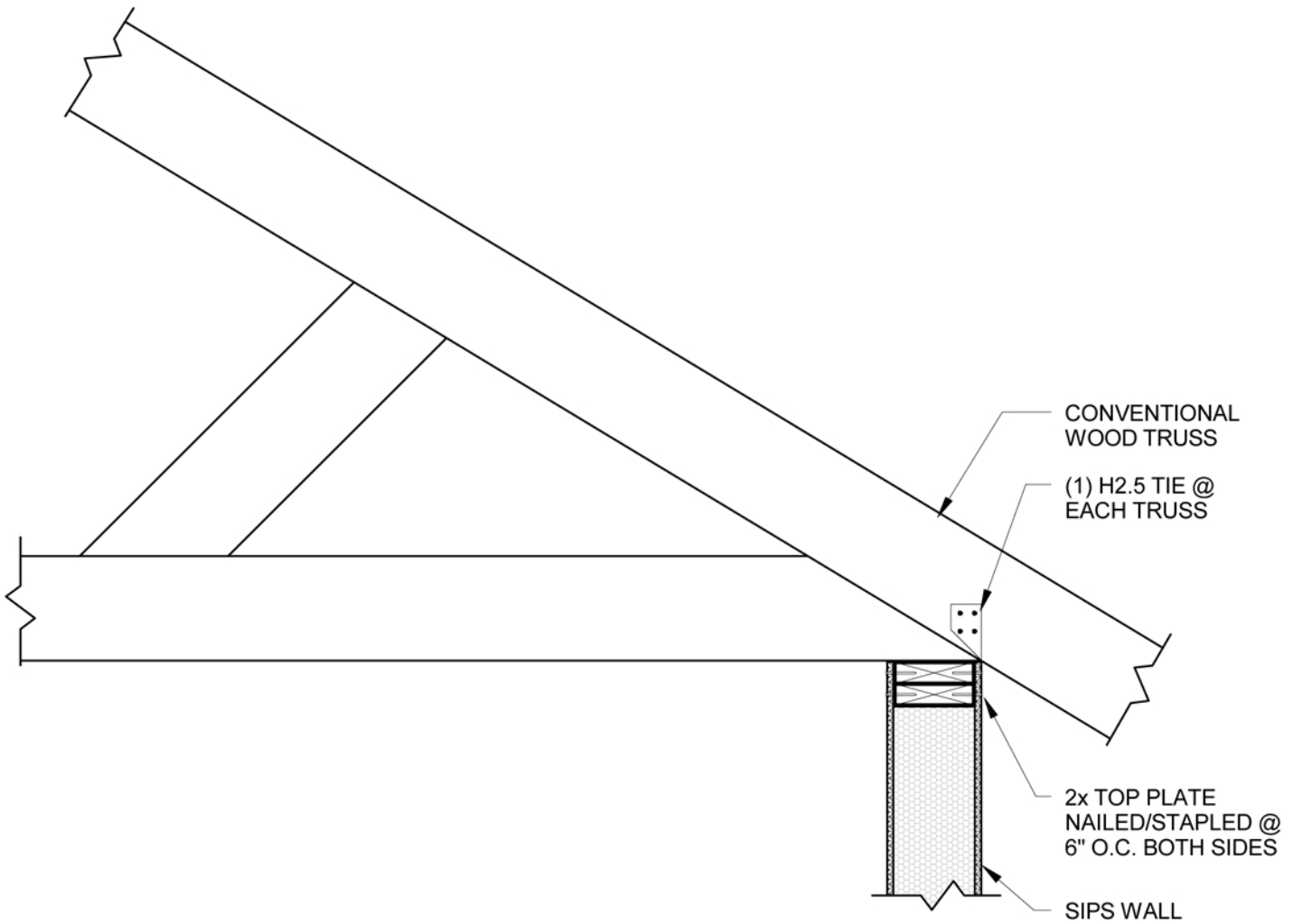
1 D40 TYP. TRUSS TO PANEL 1" = 1'-0"
