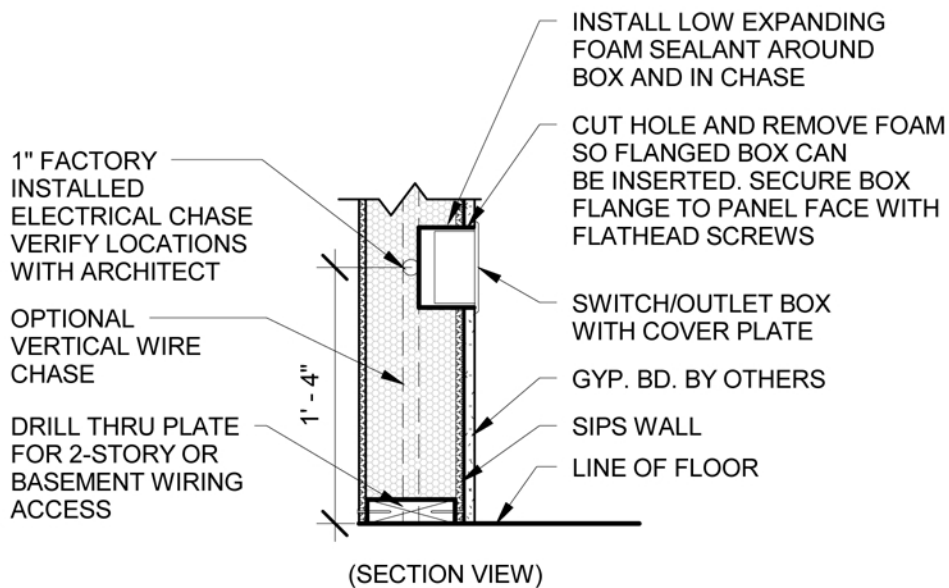
1 ELECTRICAL BOX D43 1" = 1'-0"
