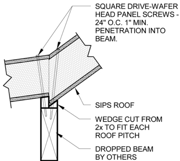
1 D44 CHANGE IN ROOF PITCH @ BEAM 1" = 1'-0"
