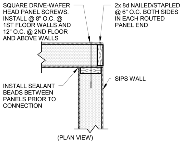
1 PANEL CORNER CONNECTION D5 1" = 1'-0"
