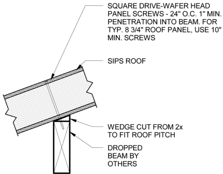
1 BEAM OFFSET @ ROOF D7 1" = 1'-0"
