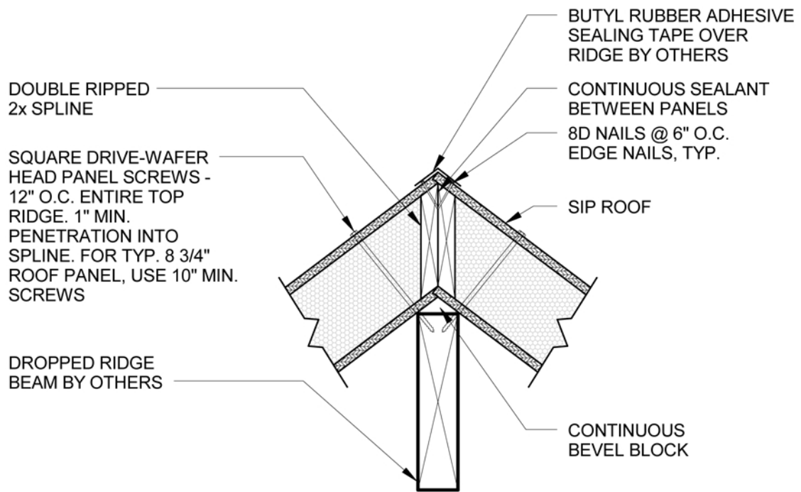
1 RIDGE BEAM @ ROOF 1" = 1'-0"
