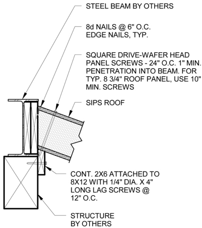
1 CONNECTION TO STEEL BEAM 1" = 1'-0"
